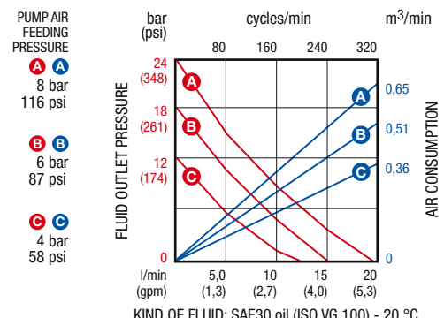
KIND OF FLUID: SAE30 oil (ISO VG 100) - 20 °C
